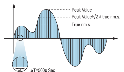
True R.M.S. Protection, Unaffected by Harmonics
