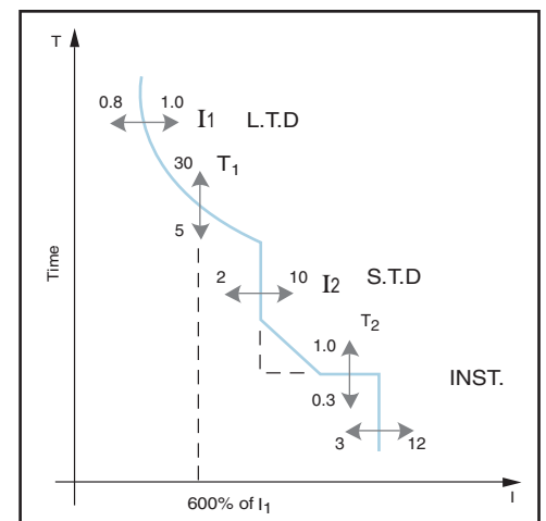
Standard Time Current Curves
